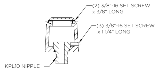
Luminaire Mounting Detail
